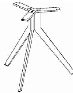
CARBON-3: 3-WAY TOP SUPPORT FRAME: 700W X 607D X 725H
